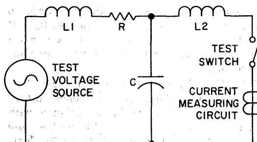
Figure 1— Suggested Test Circuit for Rated Making Duty Tests (Rated Asymmetrical Making Current Test) [See 5.4.2(1)]
